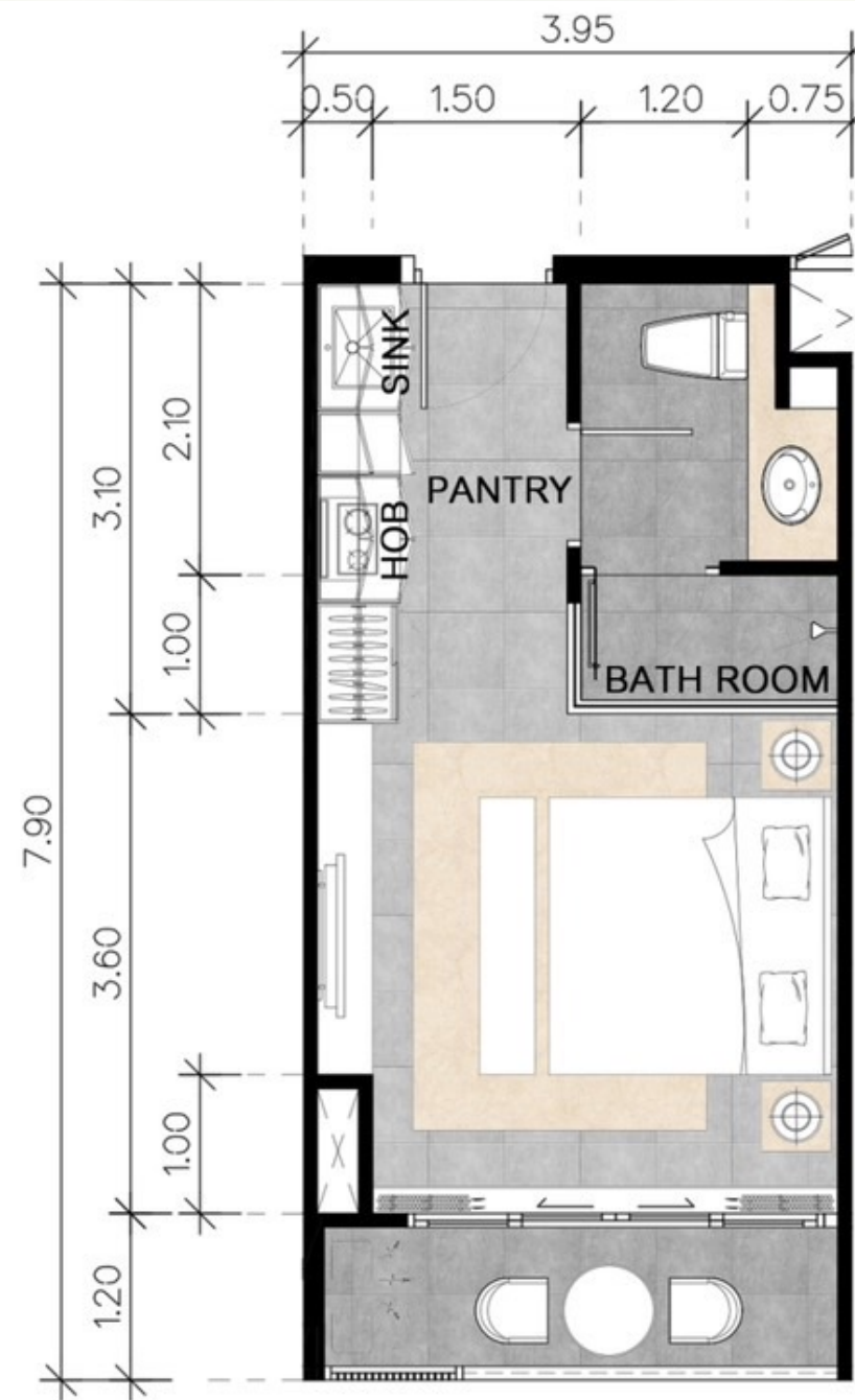
1 BEDROOM FURNITURE LAYOUT PLAN TYPE. AMS 2 TOTAL 4 UNITS AREA : 30.50 SQM.
