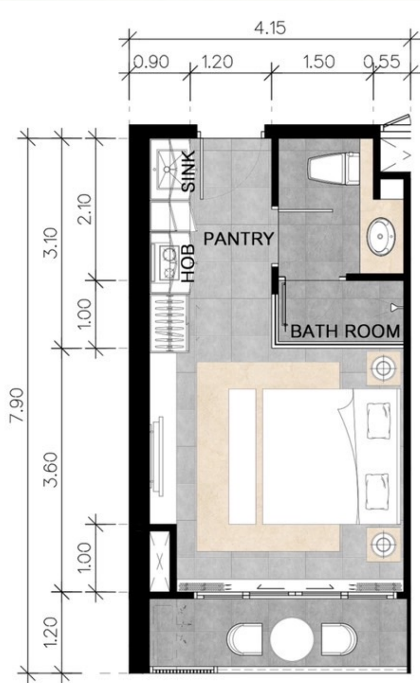
1 BEDROOM FURNITURE LAYOUT PLAN TYPE. AMS TOTAL 4 UNITS AREA : 31.54 SQM.
